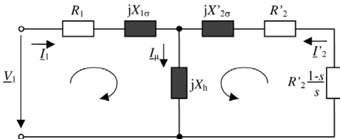
Figure 5.28 Equivalent Circuit for One Phase of an Asynchronous Machine
