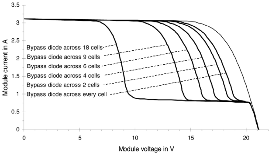
Figure 4.27 Simulation of Module Characteristics with Bypass Diodes across Different Numbers of Cells ( E = 1000 \text{ W/m}^2 , T = 300 \text{ K} )
