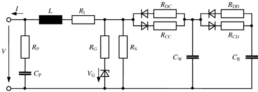
Figure 4.44 Gretsch Equivalent Circuit of a Lead–Acid Battery
