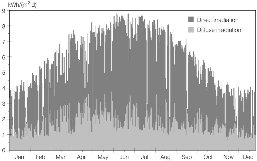
Figure 2.8 Daily Direct and Diffuse Irradiation in Cairo
