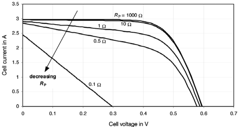
Figure 4.17 Influence of the Parallel Resistance R_p on the I-V Characteristics of a Solar Cell
