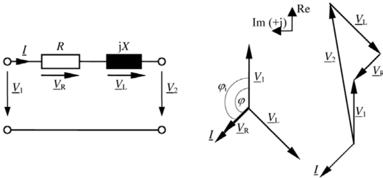
Figure 5.17 Series Connection of Resistance and Inductance with Vector Diagram
