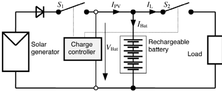
Figure 4.47 Photovoltaic Battery System with Series Charge Controller
