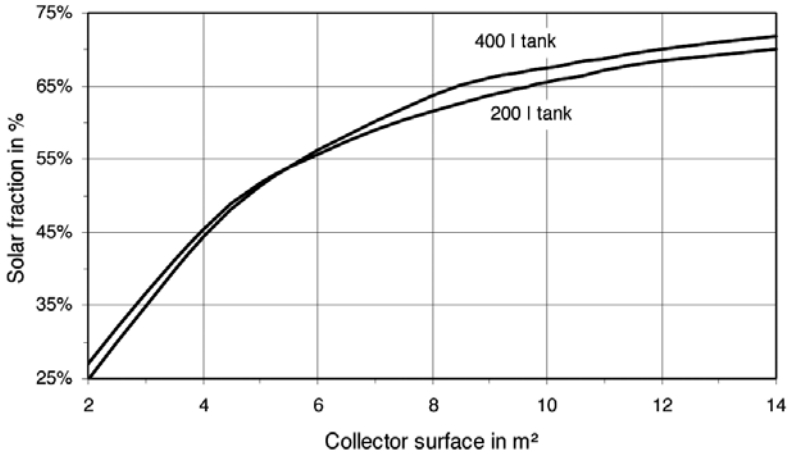
Figure 3.19 Solar Fraction as a Function of the Collector Surface: Simulation by the Software Getsolar.
