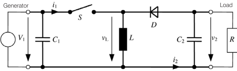
Figure 4.38 Buck–Boost Converter Circuit
