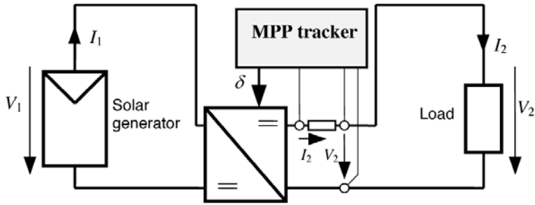
Figure 4.40 Structure of MPP Trackers
