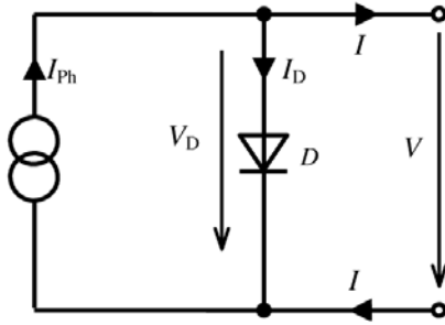
Figure 4.13 Simple Equivalent Circuit of a Solar Cell
