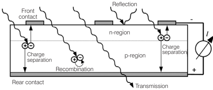
Figure 4.9 Processes in an Irradiated Solar Cell
