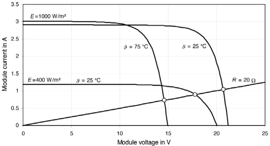
Figure 4.31 Solar Module with Resistive Load at Different Operating Conditions
