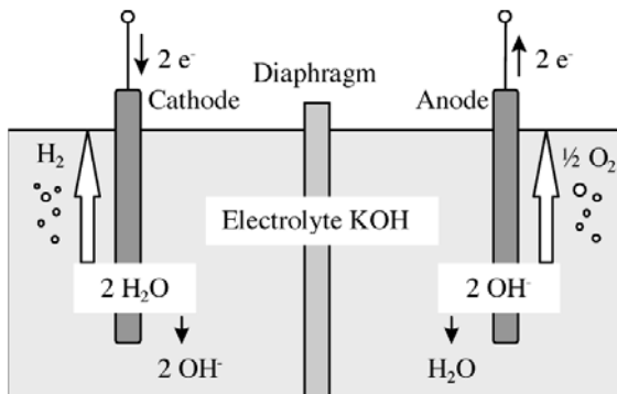
Figure 4.49 Principle of Hydrogen Electrolysis with Alkaline Electrolyte
