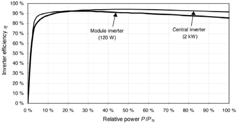
Figure 4.58 Efficiency over a Range of Relative Photovoltaic Generator Powers
