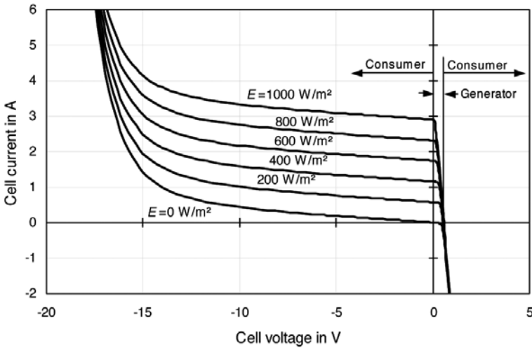
Figure 4.20 I-V Characteristics of a Polycrystalline Solar Cell over the Full Voltage Range
