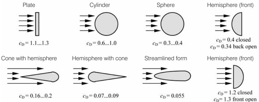
Figure 5.5 Drag Coefficients for Various Shapes
