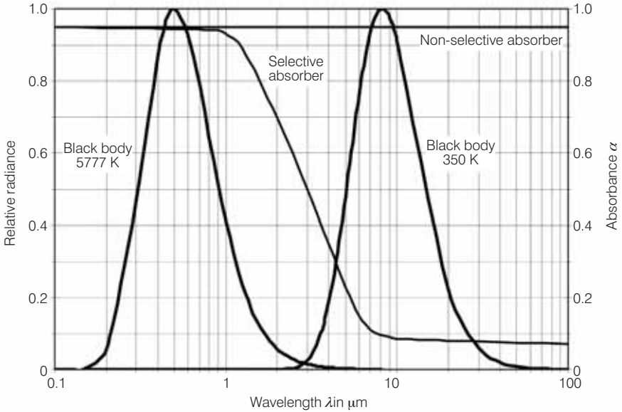
Figure 3.11 Spectra of Black Bodies at 5777 K and 350 K and the Absorptance of Selective and Non-selective Absorbers
