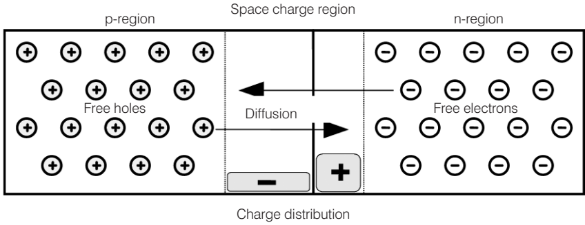
Figure 4.7 Space Charge Region Formation at a p-n Junction by Diffusion of Electrons and Holes
