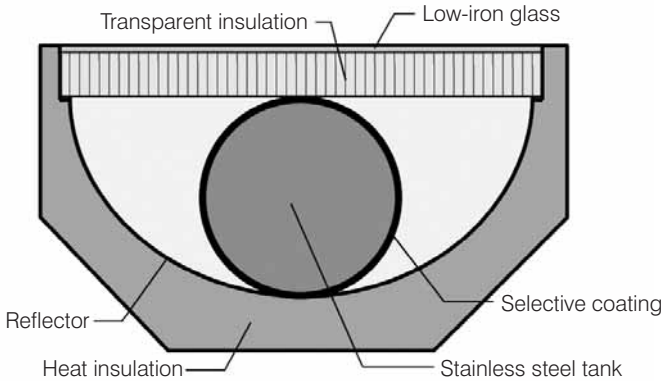
Figure 3.5 Cross-section through an Integral Collector Storage System
