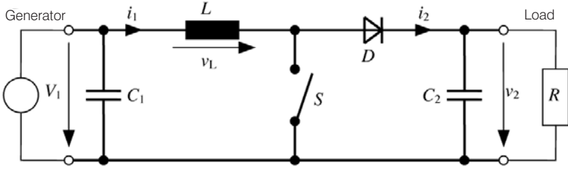
Figure 4.37 Boost Converter Circuit
