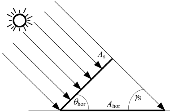
Figure 2.14 Irradiance on a Horizontal Area A_{hor} and an Area A_s Perpendicular to the Sunlight
