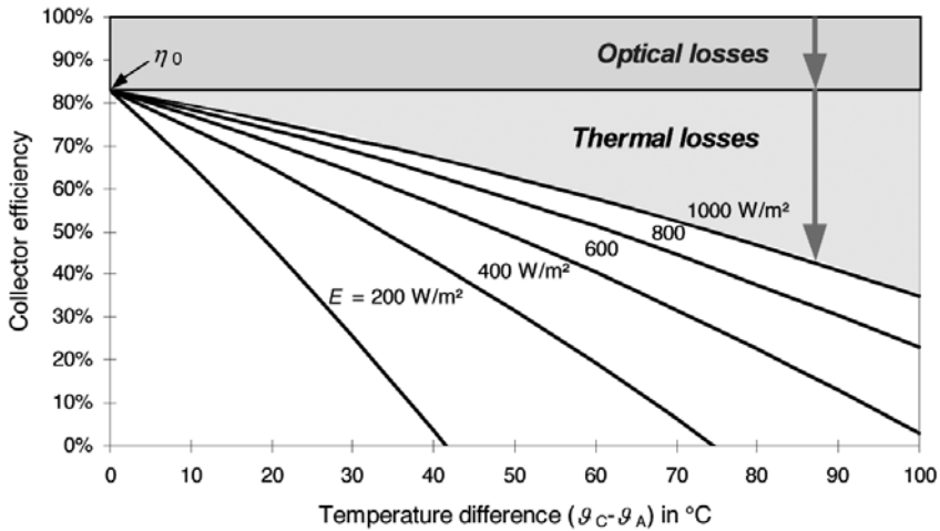
Figure 3.14 Collector Efficiencies \eta_C at Different Irradiances E and Temperature Differences \Delta\theta
