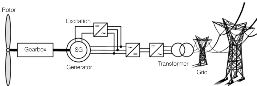
Figure 5.38 Synchronous Generator with DC Link
