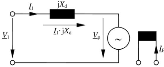
Figure 5.24 Simple Equivalent Circuit ( R_1 = 0 ) of a Cylindrical Rotor Machine for One Phase
