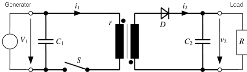
Figure 4.39 Flyback Converter Circuit
