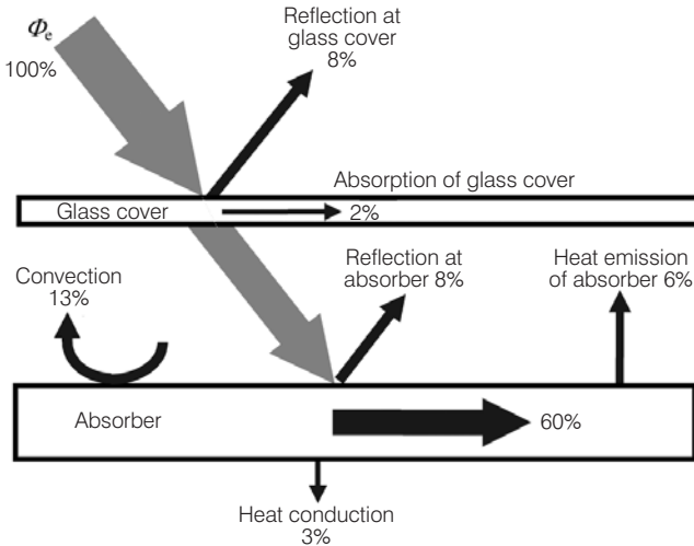
Figure 3.7 Energy Conversion in the Solar Collector and Possible Losses
