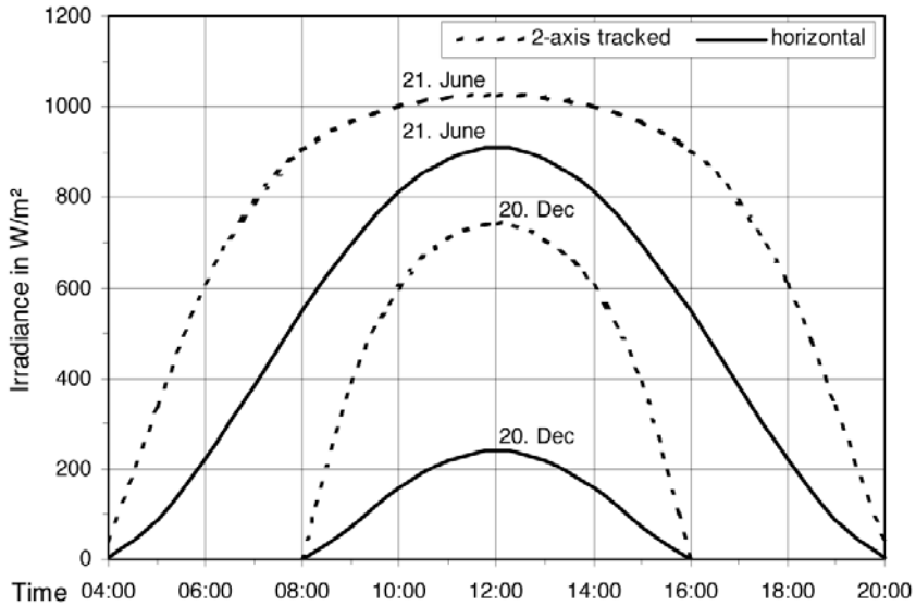
Figure 2.15 Irradiance on Horizontal and Two-axis Tracked Surfaces for Cloudless Days at a Site at 50° Latitude
