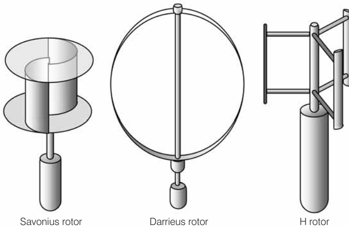
Figure 5.11 Rotors with Vertical Axes
