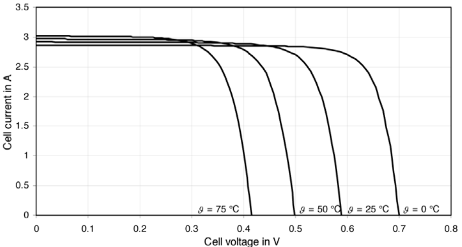
Figure 4.22 Temperature Dependence of Solar Cell Characteristics
