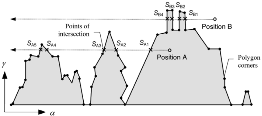
Figure 2.22 Shading Test for Two Different Positions of the Sun A and B (Position A has 5 Intersections, Position B has 4)
