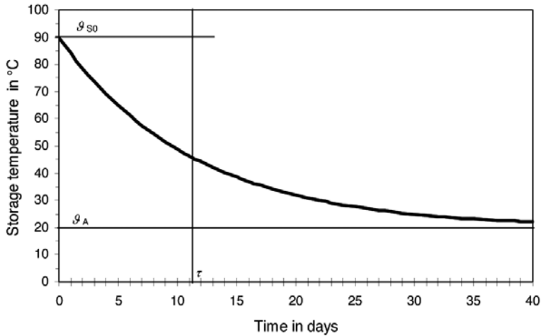
Figure 3.16 Storage Temperature \vartheta_s for a 300-litre Storage Tank without Loading or Unloading
