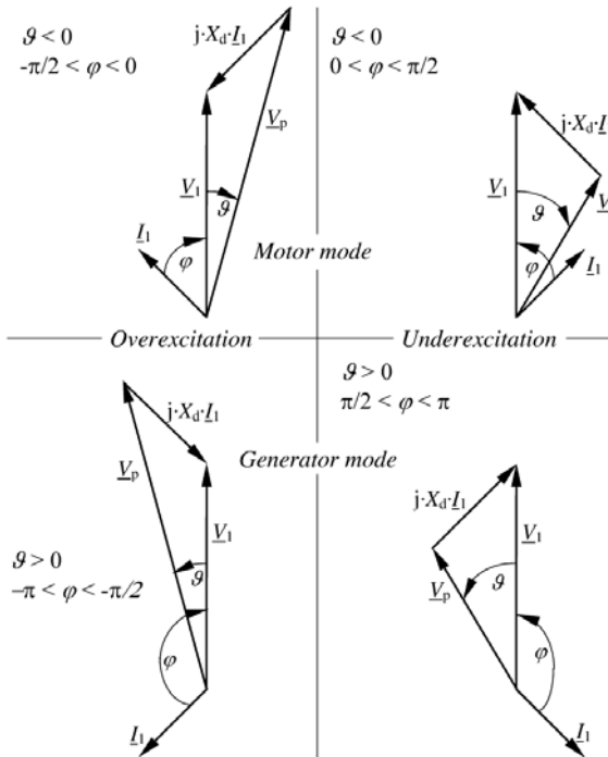
Figure 5.25 Vector Diagrams of a Synchronous Machine with Cylindrical Rotor
