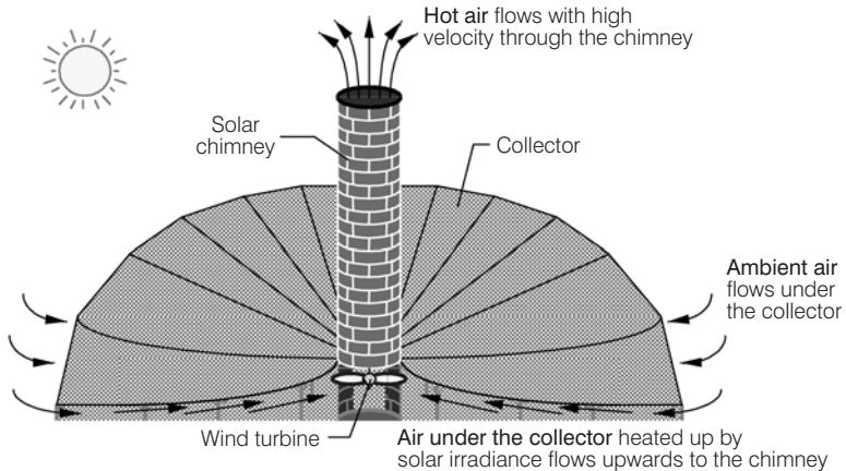
Figure 1.13 Principle of the Solar Chimney Power Plant
