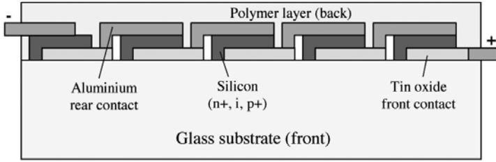
Figure 4.12 Structure of an Amorphous Silicon Solar Module
