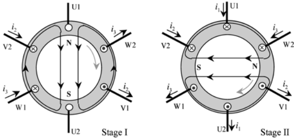
Figure 5.20 Change in the Magnetic Field at Two Different Points in Time (Stage I and Stage II) when Supplying Three Sinusoidal Currents that are Temporally Staggered by 120°
