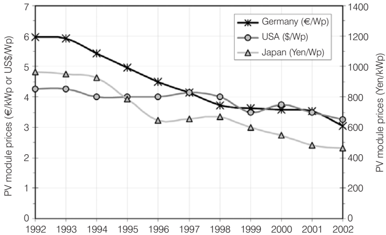
Figure 6.3 Photovoltaic Module Prices in Germany, Japan and the USA
