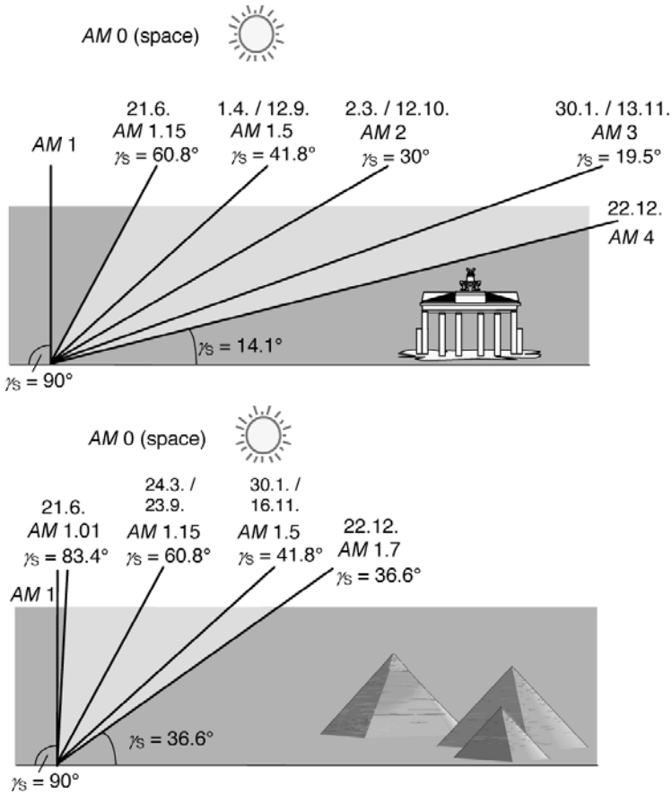
Figure 2.4 Sun Height at Solar Noon and Air Mass (AM) Values for Various Dates in Berlin (top) and Cairo (bottom)
