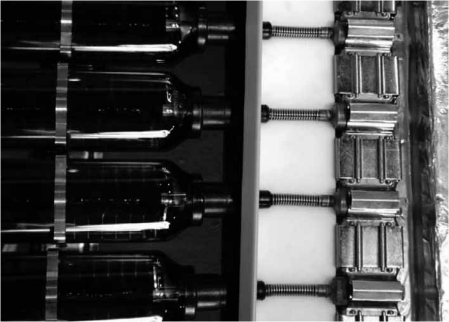
Figure 3.13 Photo of the Connections of the Evacuated Tubes to the Solar Cycle
