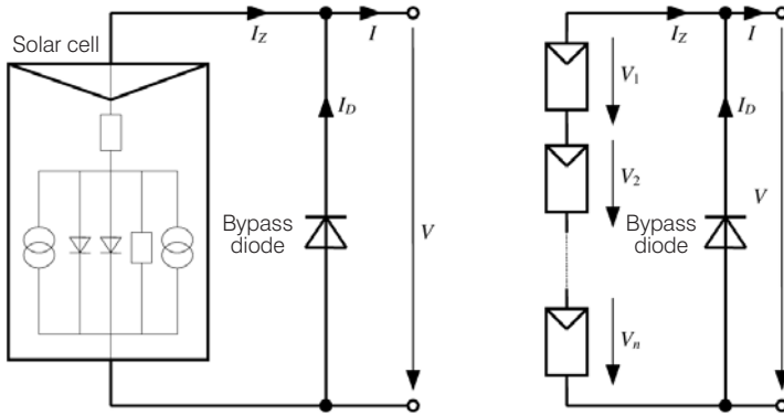
Figure 4.26 Integration of Bypass Diodes across Single Cells or Cell Strings
