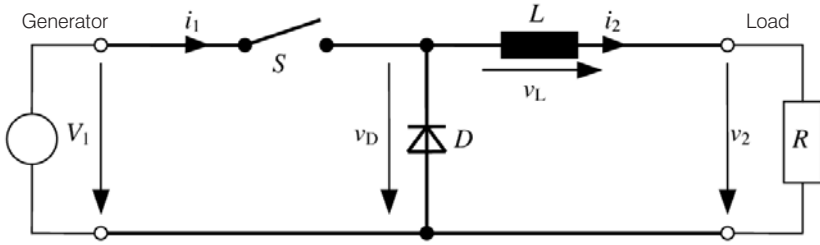
Figure 4.34 Circuit of a Buck Converter with Resistive Load
