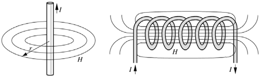
Figure 5.18 Magnetic Fields H Produced by an Electric Current in a Wire and Coil
