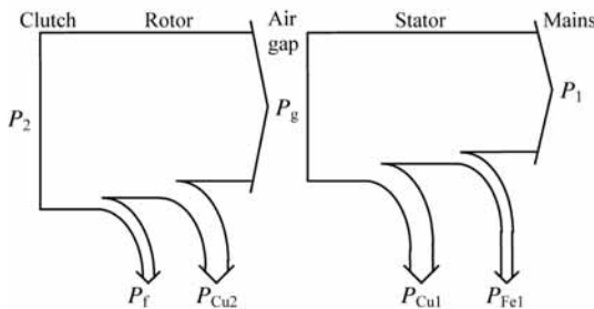
Figure 5.31 Power Balance for an Asynchronous Generator
