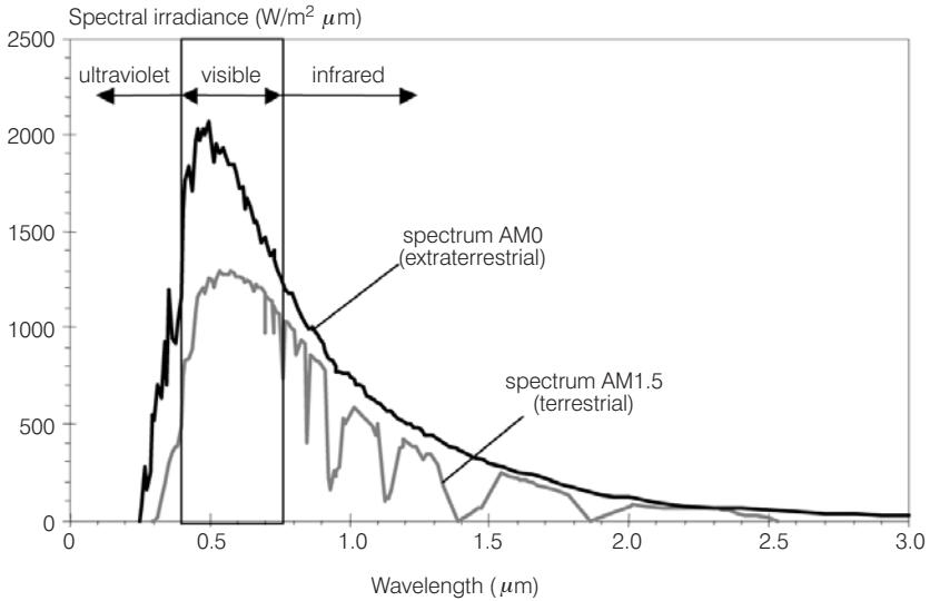
Figure 2.3 Spectrum of Sunlight
