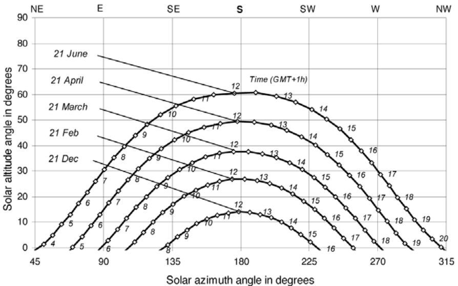
Figure 2.11 Solar Position Diagram for Berlin, Germany (52.5°N)
