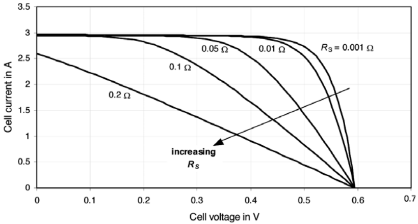
Figure 4.16 Influence of the Series Resistance R_S on the I-V Characteristics of a Solar Cell
