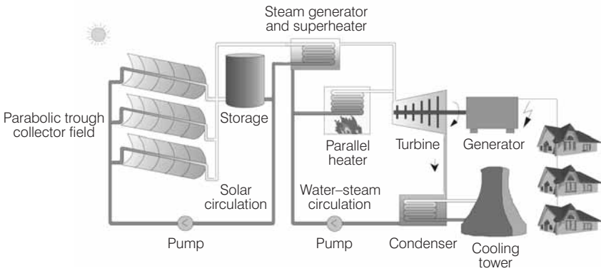
Figure 1.10 Principle of a Parabolic Trough Solar Power Plant
