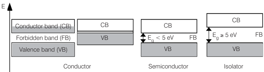
Figure 4.3 Energy Bands of Conductors, Semiconductors and Isolators
