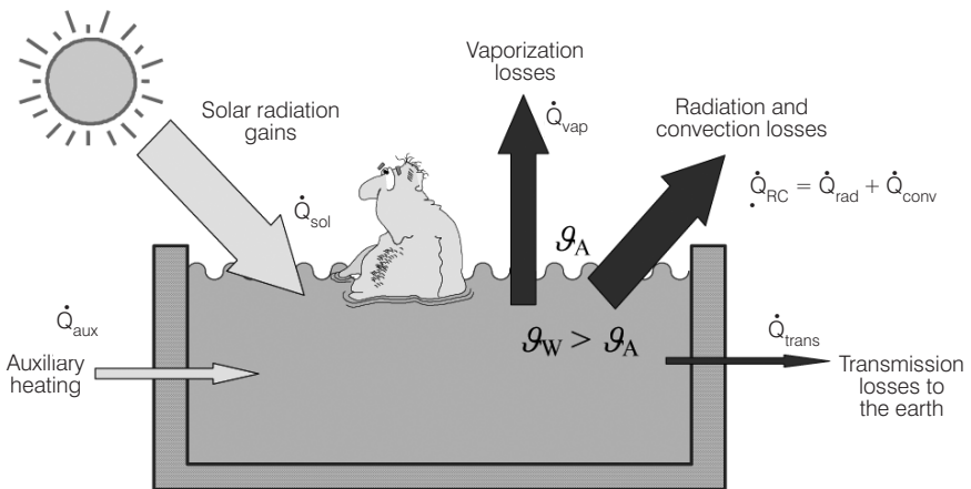
Figure 3.18 Energy Balance of a Swimming Pool
