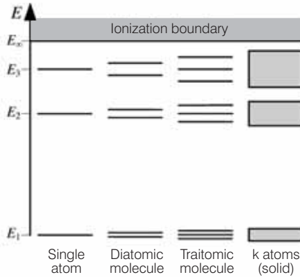
Figure 4.2 Energy States of Electrons in Atoms, Molecules and Solids
