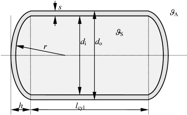
Figure 3.15 Cylindrical Hot Water Tank with Spherical Ends
