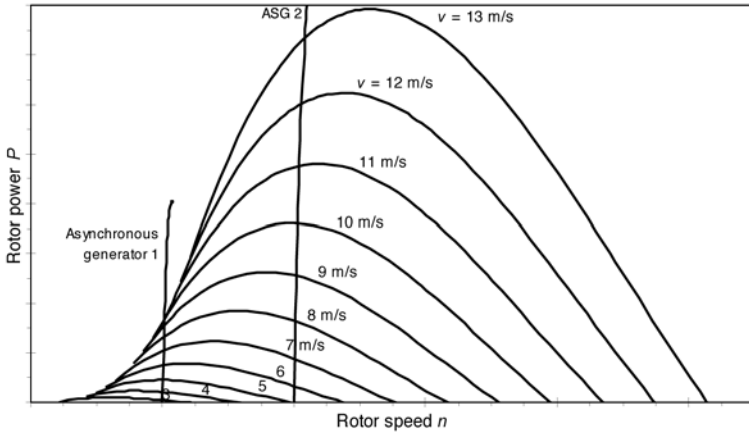
Figure 5.36 Operating Points for a Wind Turbine with Two Asynchronous Generators with Different Speeds
