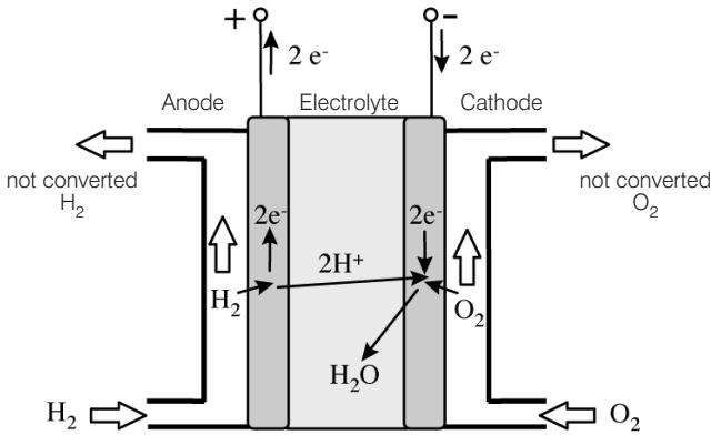
Figure 4.50 Principle of the Fuel Cell with Acid Electrolyte
