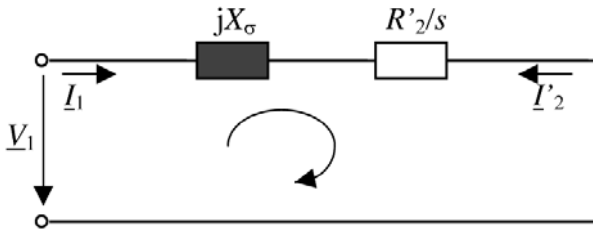
Figure 5.30 Simplified One-phase Equivalent Circuit for an Asynchronous Machine
