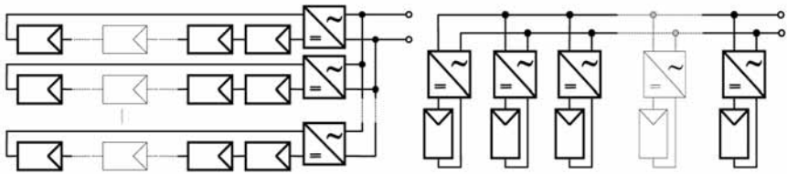
Figure 4.60 Photovoltaic Generator with String Inverters (left) and Module Inverters (right)
