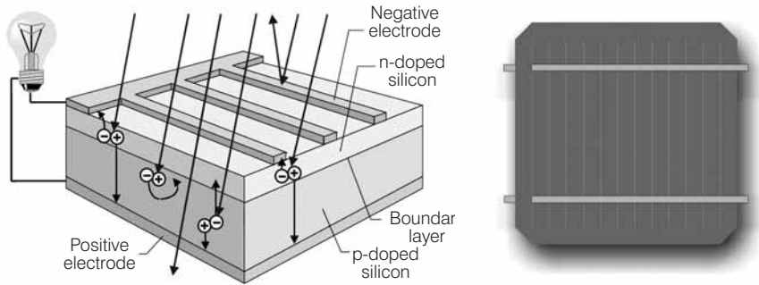
Figure 4.11 Solar Cell Structure and Front View of a Crystalline Silicon Solar Cell
