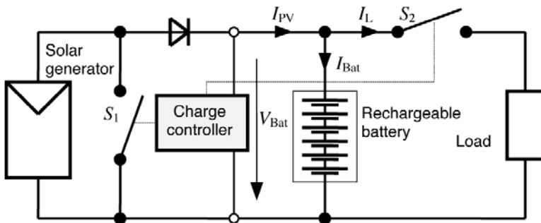
Figure 4.48 Photovoltaic Battery System with Parallel Charge Controller
