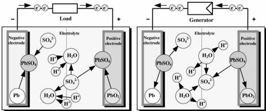
Figure 4.41 Charging and Discharging a Lead–Acid Battery
