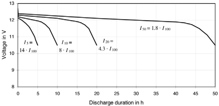
Figure 4.43 Battery Voltage as a Function of Discharge Time and Discharge Current
