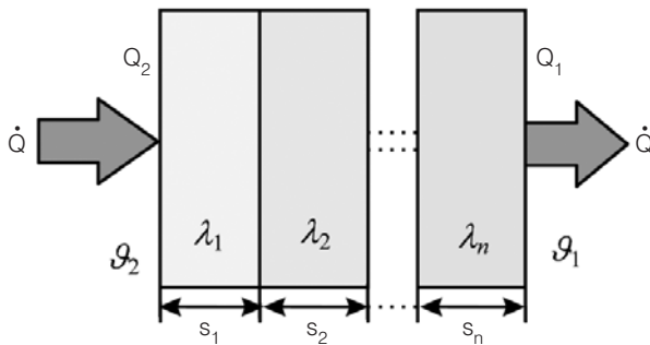
Figure 3.1 Heat Transfer through n Layers with the Same Surface Area A
