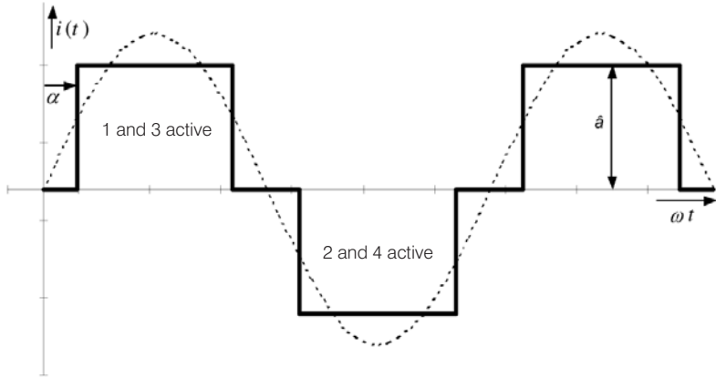
Figure 4.54 Idealized Current of a Half-controlled B2 Bridge Connection
