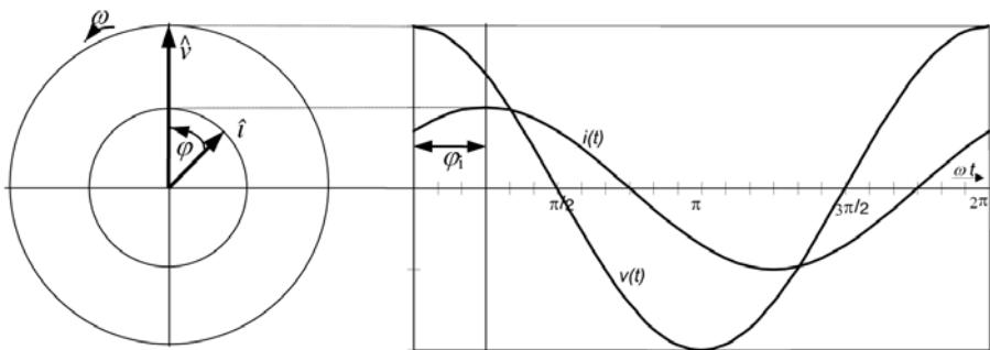
Figure 5.16 Current and Voltage as a Function of Time and Vector Diagram of the Amplitudes \hat{i} and \hat{v} ( \varphi = \pi/4 )
