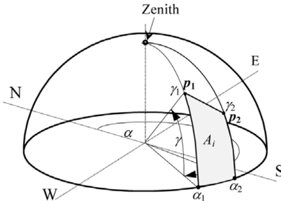
Figure 2.23 Two Points, the Horizontal Meridian and Two Polar Meridians Define the Polygon Area
