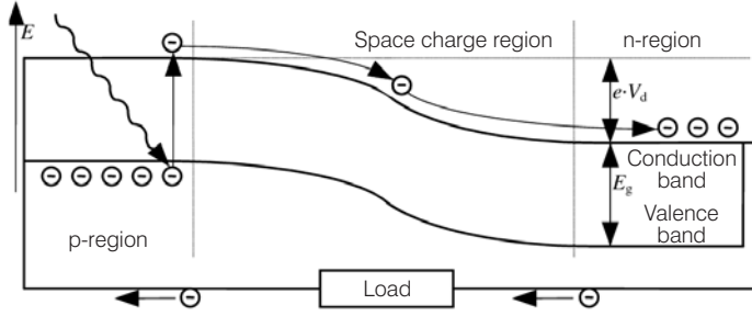
Figure 4.8 Solar Cell Principle with Energy Band Model
