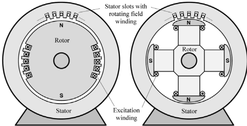
Figure 5.23 Cross-section through a Synchronous Machine; Left: Cylindrical Rotor, Right: Salient-pole Rotor
