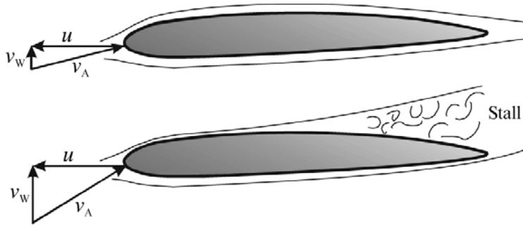
Figure 5.14 Stall Effect at Higher Wind Speeds
