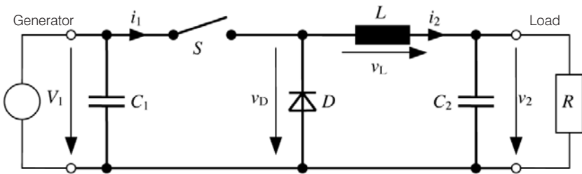
Figure 4.36 Buck Converter with Capacitors
