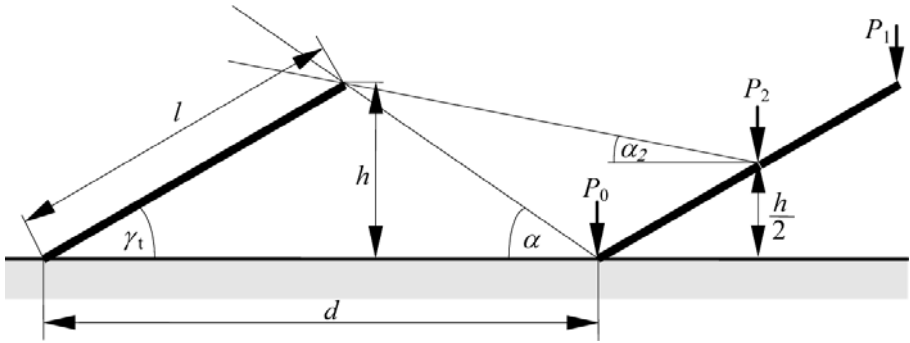
Figure 2.24 Dimensions of Solar Energy Systems and Support Structure Rows
