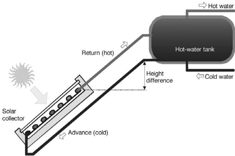
Figure 3.3 Schematic of a Thermosyphon System
