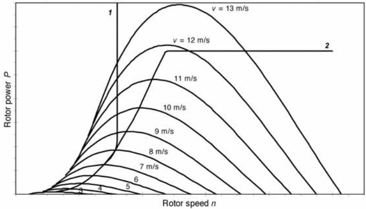
Figure 5.39 Operating Points for a Variable-Speed Wind Generator with Power Limited by Constant Speed (1) or by a Converter (2)
