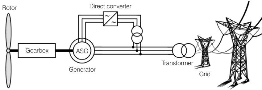
Figure 5.41 Double-fed Asynchronous Generator with Direct Converter
