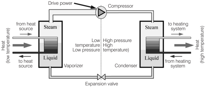
Figure 1.19 Principle of a Compression Heat Pump
