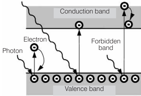
Figure 4.4 The Lifting of Electrons from the Valence Band to the Conduction Band Caused by Light Energy in a Semiconductor (Inner Photo Effect)
