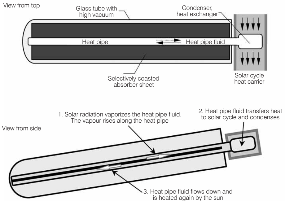
Figure 3.12 Assembly and Function of the Evacuated Tube Collector with Heat Pipe
