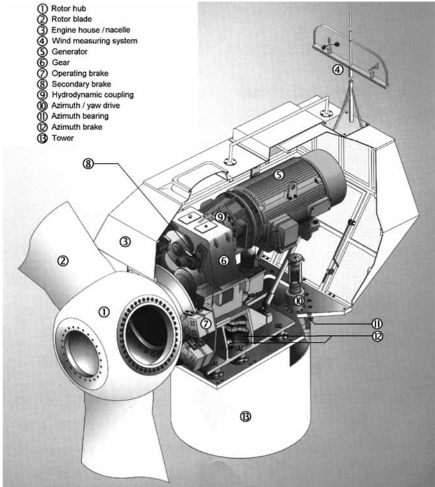
Figure 5.12 Section through the Stall-controlled TW600 Wind Generator (600 kW Change-pole Asynchronous Generator, 43 m Rotor Diameter, 50–70 m Hub Height)
