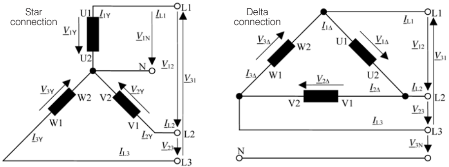
Figure 5.22 Principle of Star and Delta Connections
