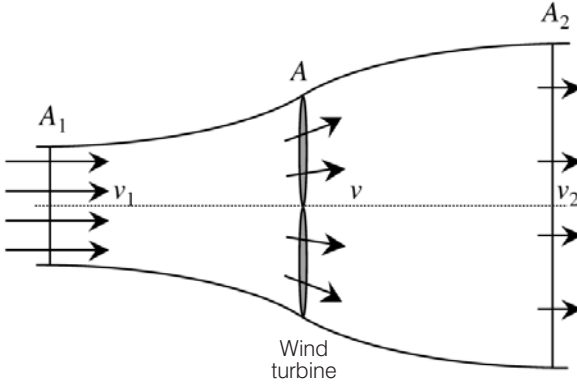
Figure 5.4 Idealized Change of Wind Speed at a Wind Turbine
