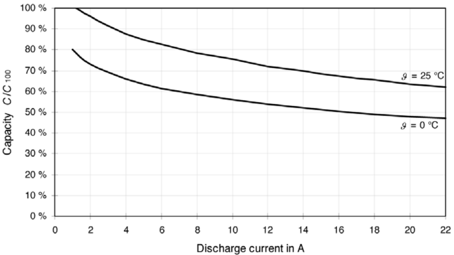
Figure 4.42 Usable Capacity Related to C_{100} = 100 A h of a Lead–Acid Battery as a Function of the Discharge Current and Temperature
