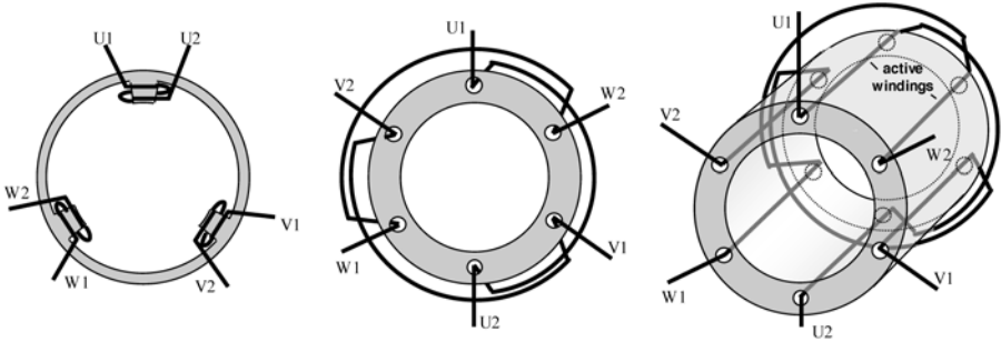
Figure 5.19 Left: Cross-section through a Stator with Three Coils Staggered by 120° for the Generation of a Rotating Field (Concentrated Winding); Middle: Cross-section; Right: Three-dimensional Drawing of an Integrated Rotating Field Winding (Distributed Winding)
