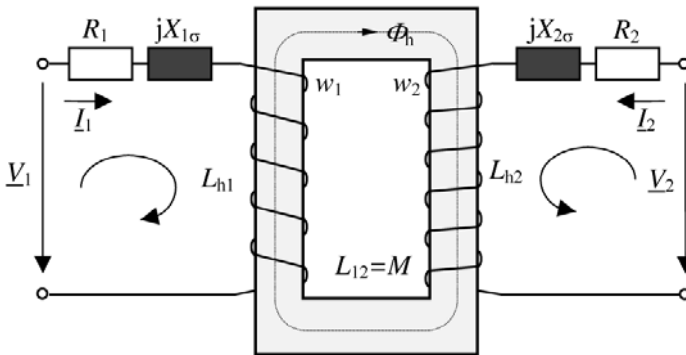
Figure 5.27 Ideal Transformer with Resistances and Reactances
