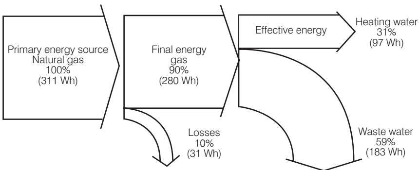
Figure 1.2 Energy Conversion Chain and Losses for Water Heating with a Gas Cooker
