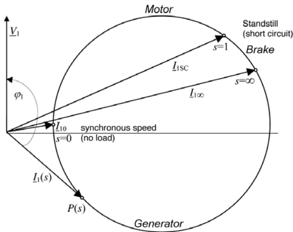
Figure 5.29 Circle Diagram for the Estimation of the Stator Current According to Heyland and Ossanna
