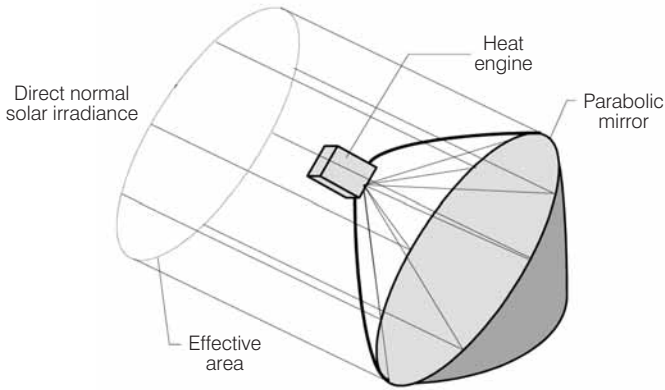
Figure 1.12 Principle of a Dish–Stirling System
