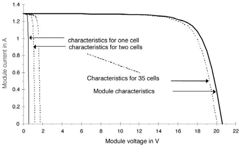
Figure 4.24 Construction of Module Characteristics with 36 Cells (Irradiance E = 400 \text{ W/m}^2 , T = 300 \text{ K} )
