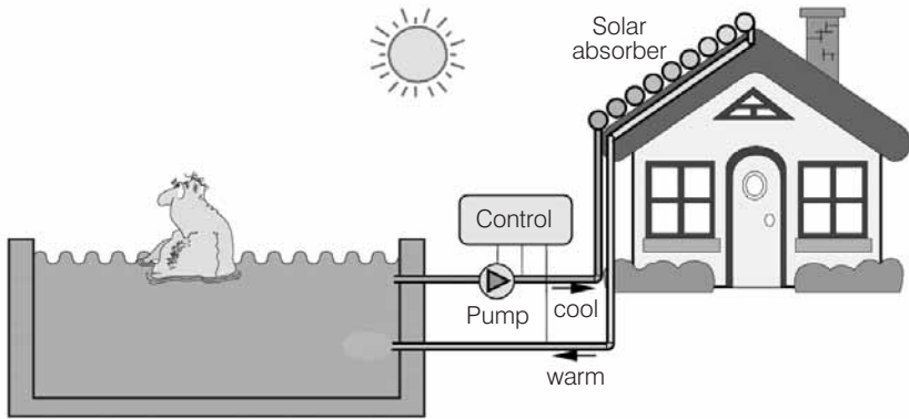
Figure 3.2 Principle of Solar Thermal Swimming Pool Heating
