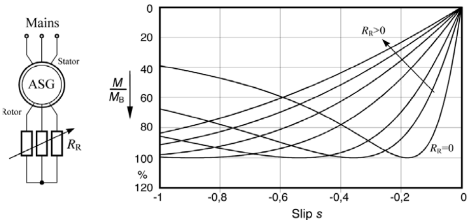
Figure 5.34 Torque Characteristics as a Function of Slip s with Variation of the Rotor Resistance R_R
