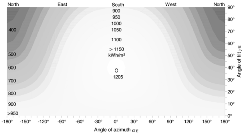
Figure 2.16 Annual Irradiation on Various Inclined Surfaces in Berlin (52.5°N)
