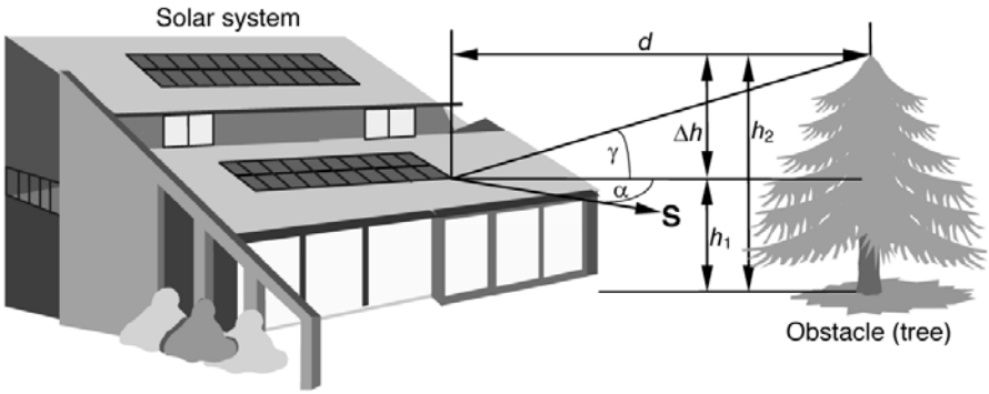
Figure 2.18 Definition of the Obstacle Height Angle and Obstacle Azimuth Using a Freely Chosen Point of Reference
