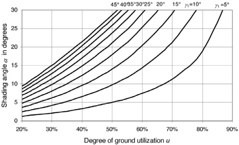
Figure 2.25 Shading Angle \alpha as a Function of the Degree of Ground Utilization u and the Surface Tilt Angle \gamma_t
