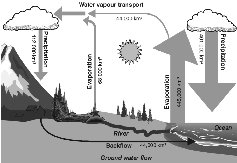
Figure 1.14 Principle of the Global Water Cycle
