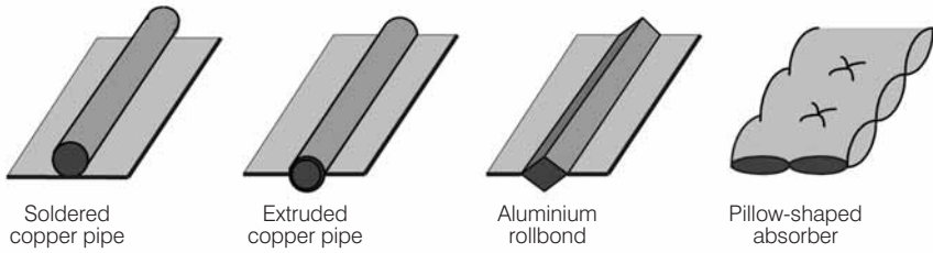
Figure 3.9 Various Designs of Solar Absorber
