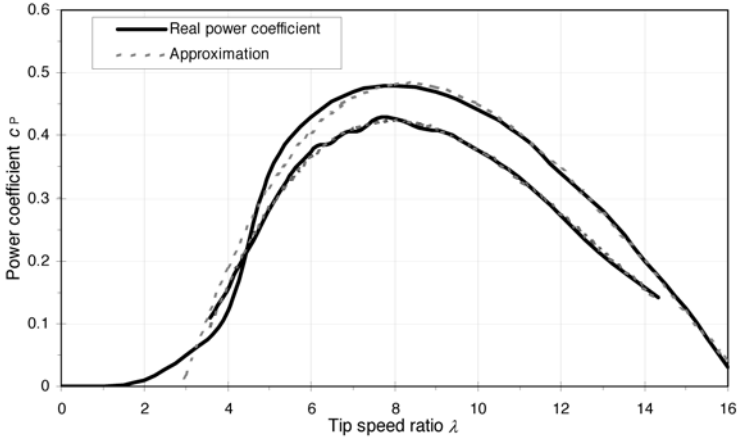
Figure 5.10 Power Coefficients and Approximations using Third-degree Polynomials
