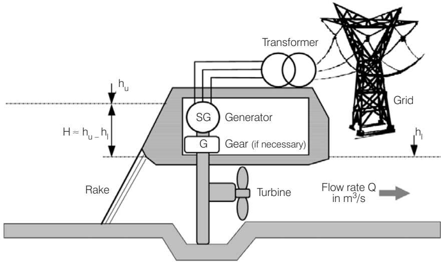
Figure 1.15 Principle of a Hydro-electric Power Plant
