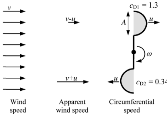
Figure 5.6 Model of Cup Anemometer for the Calculation of Power
