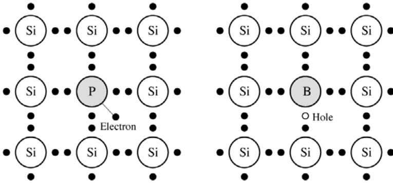
Figure 4.6 Defect Conduction for n-type and p-type Doped Silicon
