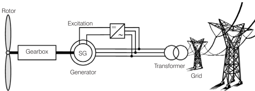
Figure 5.37 Synchronous Generator with Direct Mains Coupling
