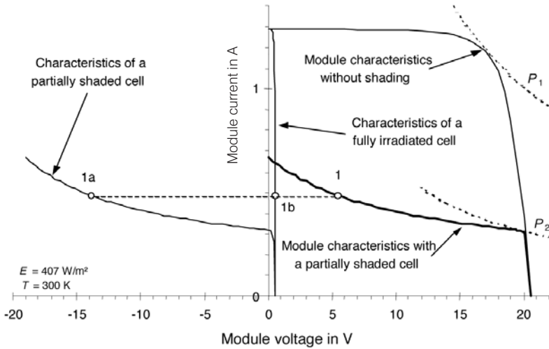
Figure 4.25 Construction of Module Characteristics with a 75 per cent Shaded Cell
