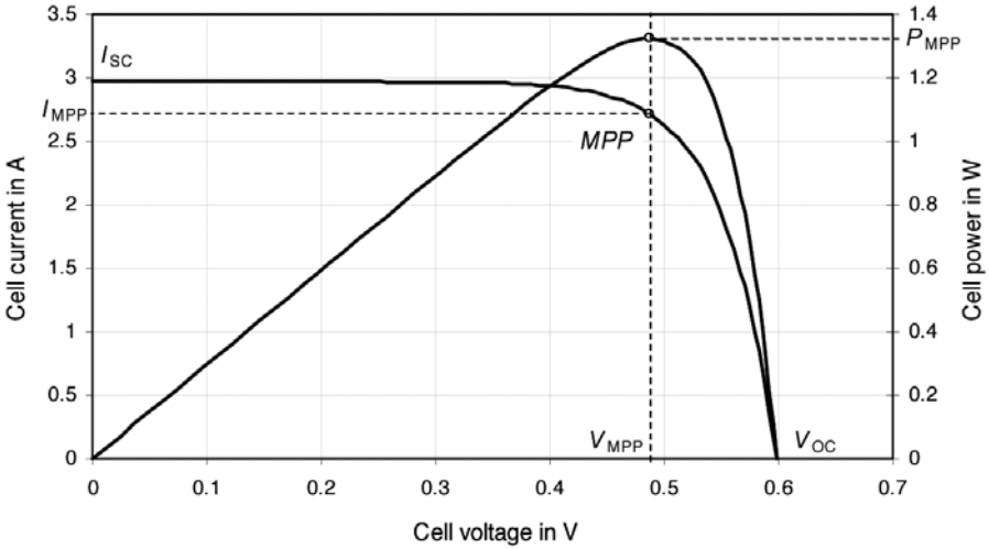
Figure 4.21 I-V and P-V Solar Cell Characteristics with Maximum Power Point (MPP)
