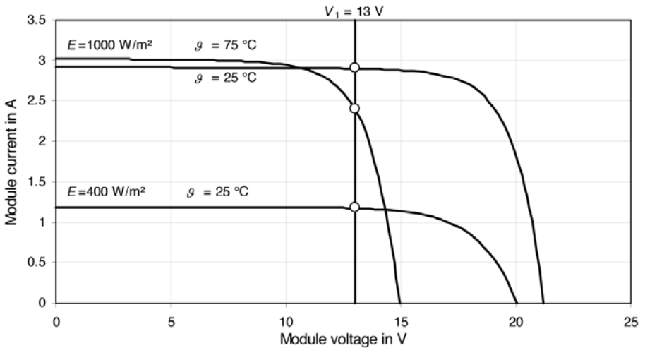
Figure 4.33 Solar Module with Constant Voltage Load for Three Different Operating Conditions
