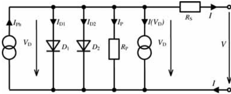
Figure 4.19 Two-diode Equivalent Circuit with Second Current Source to Describe the Solar Cell Breakdown at Negative Voltages
