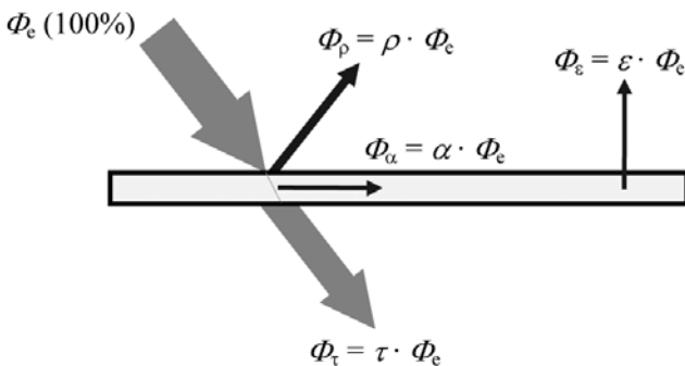
Figure 3.8 Processes at the Collector Front Glass Cover
