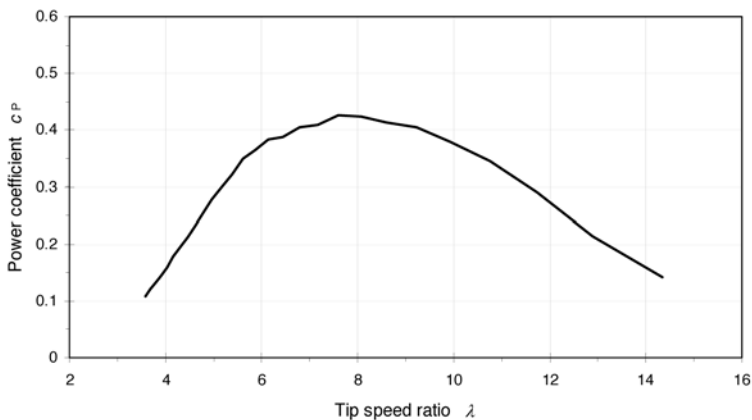
Figure 5.9 Power Coefficient c_p as a Function of the Tip Speed Ratio \lambda for the Vestas V44-600-kW Wind Generator
