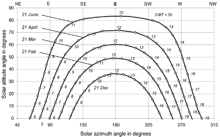
Figure 2.12 Solar Position Diagram for Cairo, Egypt ( 30.1^\circ\text{N} )
