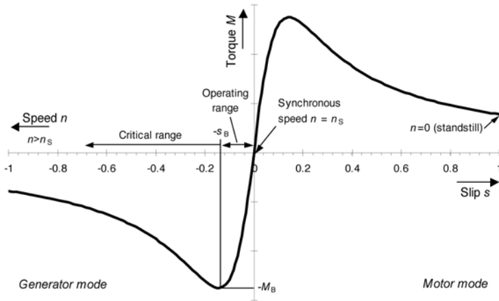
Figure 5.32 Speed-torque Characteristics for an Asynchronous Machine
