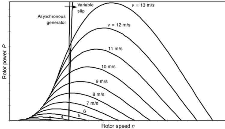
Figure 5.35 Operating Points for a Wind Turbine with Asynchronous Generator that is Directly Coupled to the Mains
