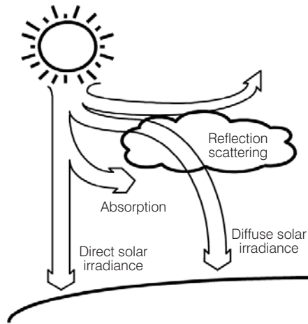
Figure 2.6 Sunlight Passing Through the Atmosphere
