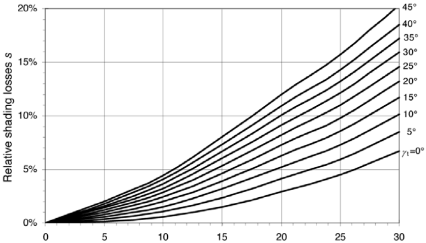
Figure 2.26 Relative Shading Losses s as a Function of the Shading Angle \alpha and Surface Tilt Angle \gamma_t in Berlin ( 52.5^\circ\text{N} )
