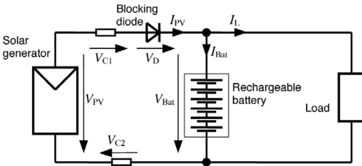
Figure 4.45 Simple Photovoltaic System with Battery Storage
