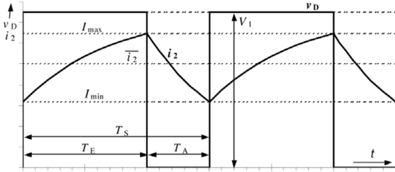
Figure 4.35 Current i_2 and Voltage v_D for a Buck Converter
