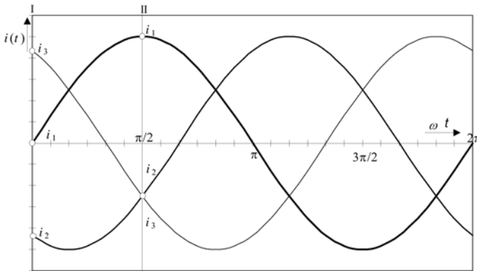
Figure 5.21 Three-phase Currents to Generate a Rotating Field
