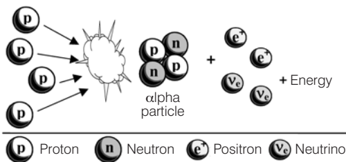
Figure 2.1 Fusion of Four Hydrogen Nuclei to Form One Helium Nucleus (Alpha Particle)
