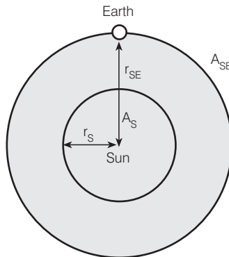
Figure 2.2 The Radiant Power through the Surface of a Sphere with Radius r_{SE} is the Same as through the Surface of the Sun
