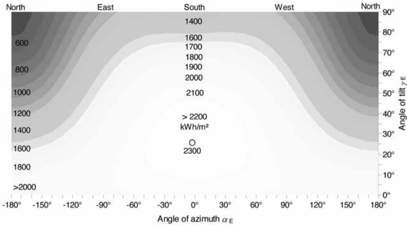
Figure 2.17 Annual Irradiation on Various Inclined Surfaces in Cairo (30.1°N)
