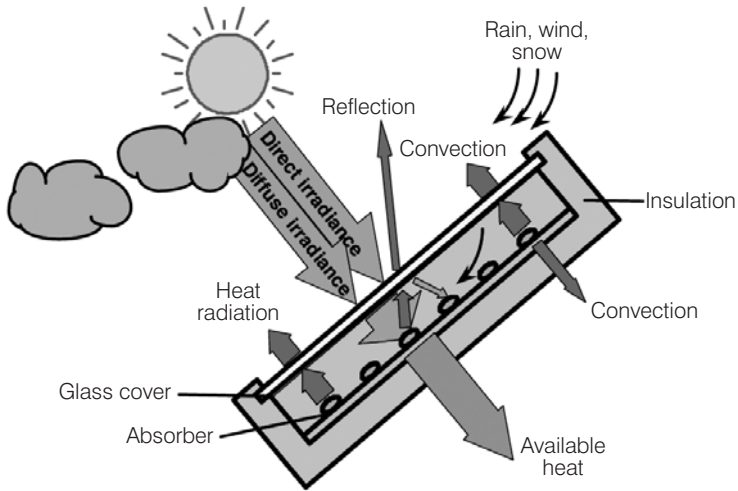
Figure 3.6 Processes in a Flat-plate Collector
