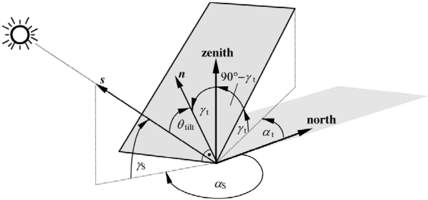
Figure 2.13 Definition of the Solar Angle of Incidence on a Tilted Surface
