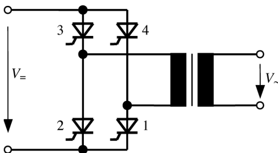
Figure 4.53 Two-pulse Bridge Connection (B2)
