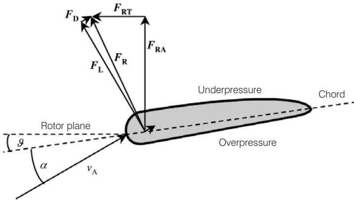
Figure 5.8 Ratio of the Forces for a Lift Device
