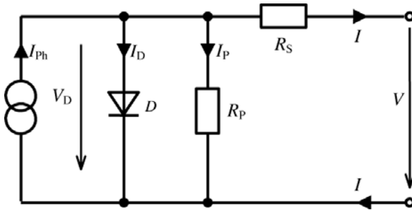
Figure 4.15 Extended Equivalent Circuit of a Solar Cell (One-diode Model)
