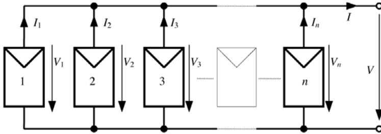
Figure 4.29 Parallel Connection of n Solar Cells
