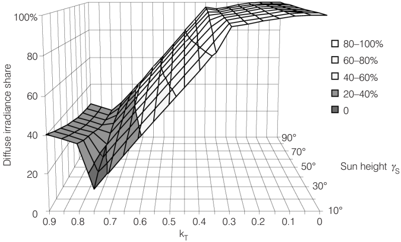
Figure 2.9 Diffuse Irradiance Component as a Function of k_T and \gamma_S
