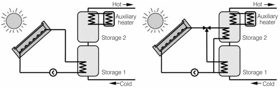
Figure 3.17 Collector Systems with Two Storage Tanks
