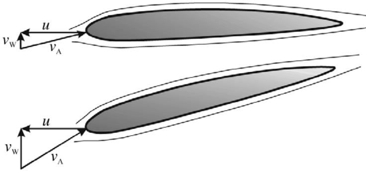
Figure 5.15 Rotor Blade Positions for Different Wind Speeds for a Pitch-controlled System
