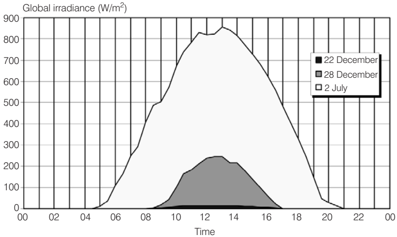
Figure 2.5 Global Irradiance throughout the Day in Karlsruhe (Germany) for 2 July and 22 and 28 December 1991
