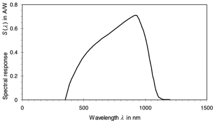
Figure 4.10 Spectral Response of a Solar Cell
