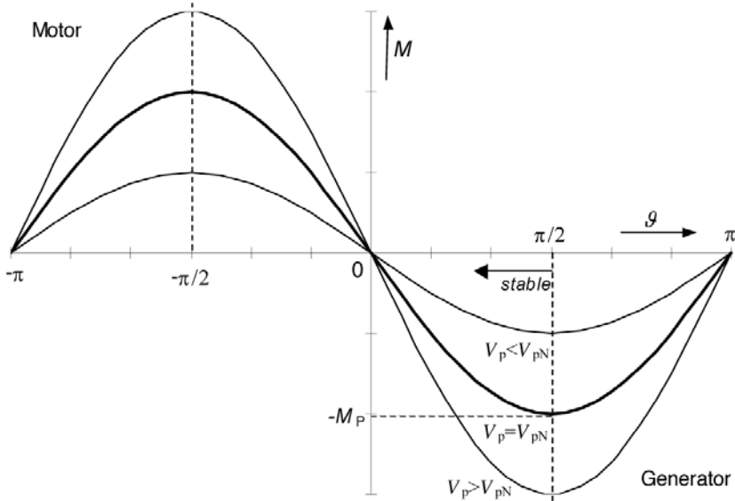
Figure 5.26 Curve of the Torque of a Synchronous Machine with Cylindrical Rotor as a Function of the Load Angle \vartheta and the Internal Voltage V_p
