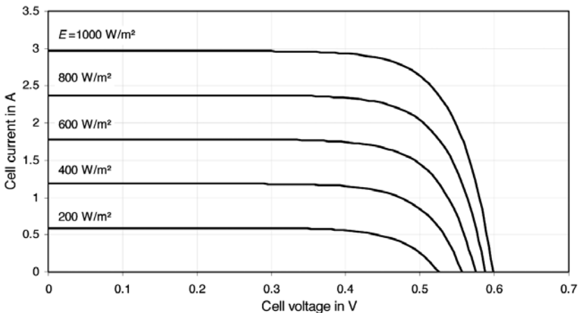
Figure 4.14 Influence of the Irradiance E on the I - V Characteristics of a Solar Cell
