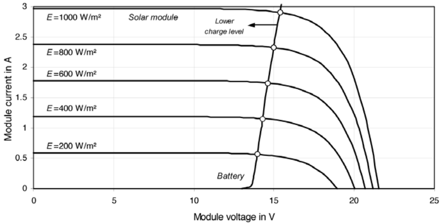
Figure 4.46 Operating Points of a Solar Module Connected to Battery Storage with a Blocking Diode and 0.1 \Omega Cable Resistance without Load
