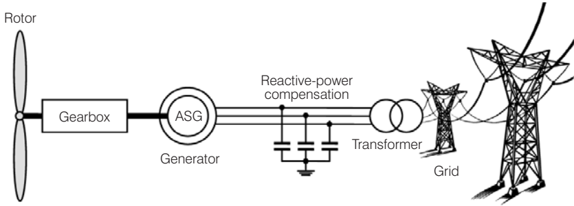
Figure 5.33 Asynchronous Generator with Direct Mains Coupling
