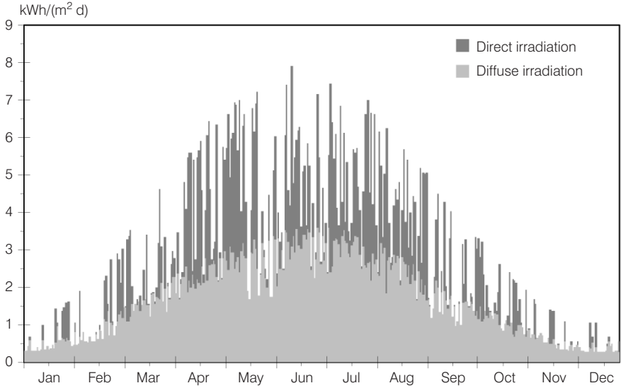
Figure 2.7 Daily Direct and Diffuse Irradiation in Berlin
