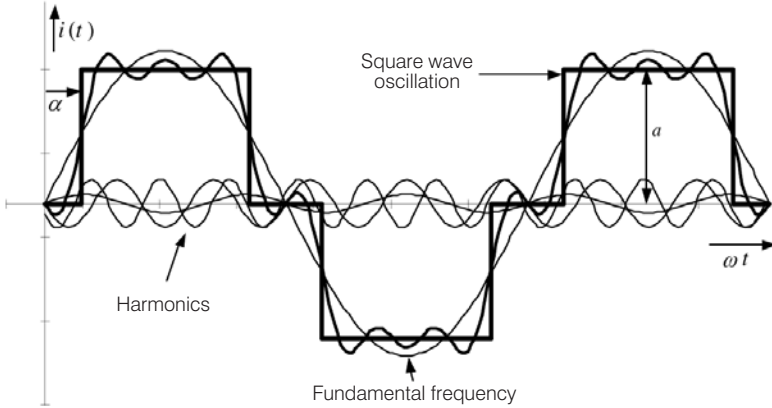
Figure 4.55 Construction of a Square-wave Oscillation from Different Sinusoidal Harmonics
