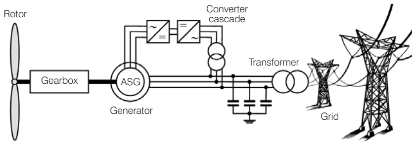
Figure 5.40 Variable Speed Asynchronous Generator with Converter Cascade
