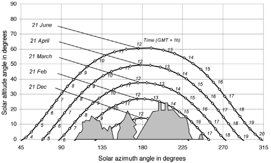
Figure 2.21 Solar Position Diagram of Berlin with an Approximation of the Surroundings
