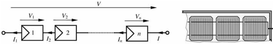
Figure 4.23 Series Connection of Photovoltaic Solar Cells (left: Electrical Symbols, Currents and Voltages; right: Top View of a Part of a Module with Crystalline Cells)
