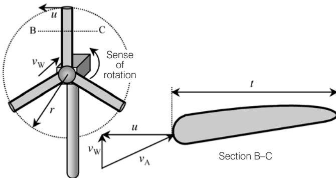
Figure 5.7 Apparent Wind Speed v_A Resulting from the Real Wind Speed v_W and Rotor Motion
