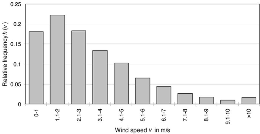
Figure 5.1 Wind Speed Distribution for Karlsruhe in Inland Germany in 1991/1992
