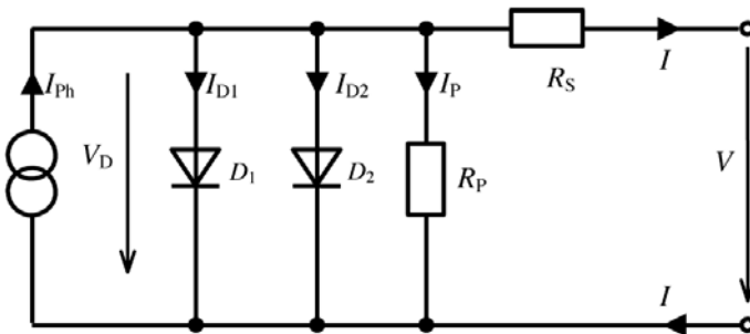
Figure 4.18 Two-diode Model of a Solar Cell
