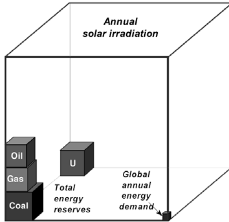
Figure 1.9 Energy Cubes; the Annual Solar Irradiation Exceeds Several Times the Total Global Energy Demand and All Fossil Energy Reserves
