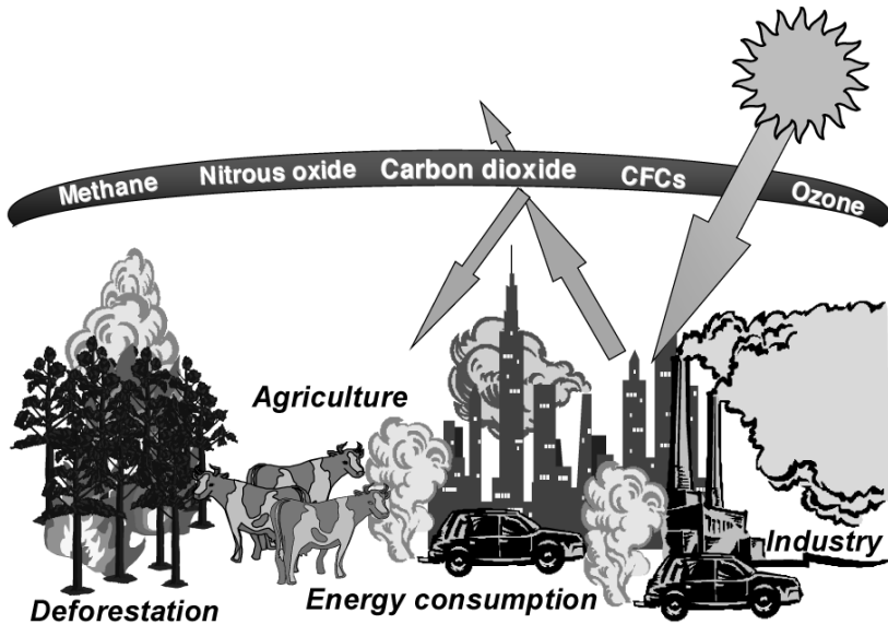
Figure 1.6 Origin of the Anthropogenic (Human-induced) Greenhouse Effect
