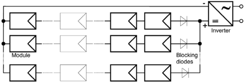
Figure 4.59 Photovoltaic System with Parallel Strings and Central Inverter
