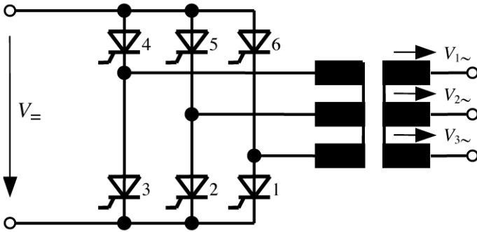
Figure 4.56 Six-pulse Bridge Inverter (B6)
