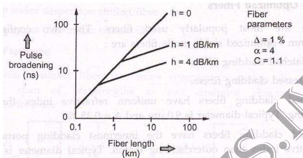
Fig. 2.8.1 Mode coupling effects on pulse broadening
