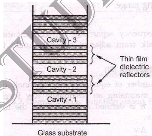
Fig. 7.7.1 Three cavity filter
