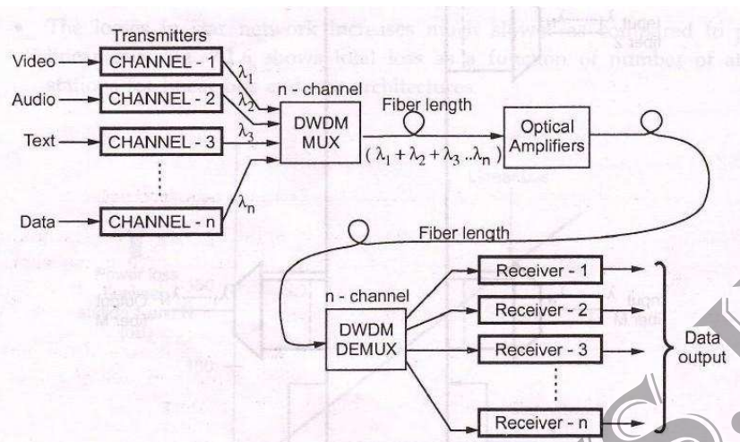
Fig. 7.2.1 DWDM system
