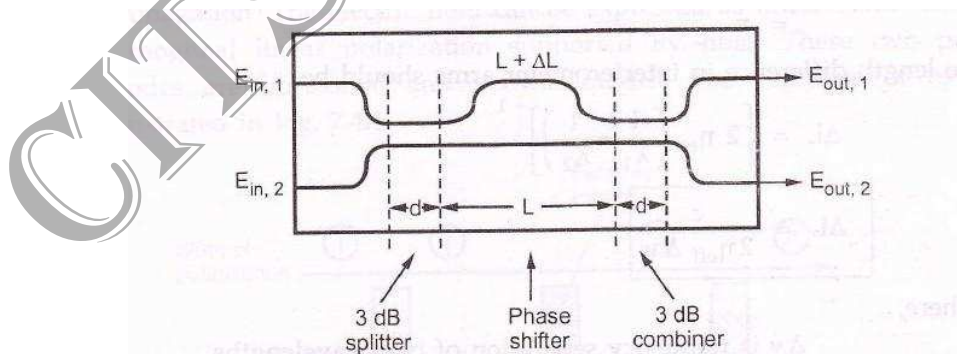
Fig. 7.3.1 Layout of 2 \times 2 passive Mach-Zehnder Interferometer
