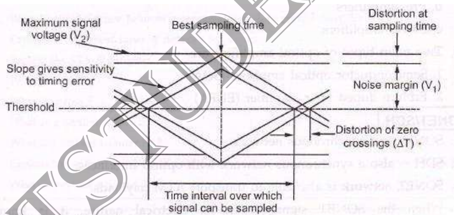
Fig. 8.7.4 Simplified Eye-diagram with key performance parameters
