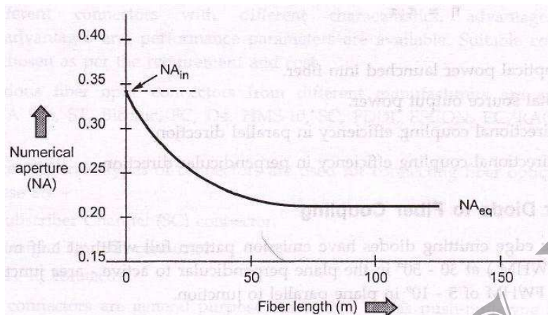
Fig. 4.5.1 Change in NA as a function of fiber length
