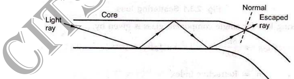
Fig. 2.4.1 Bending loss
