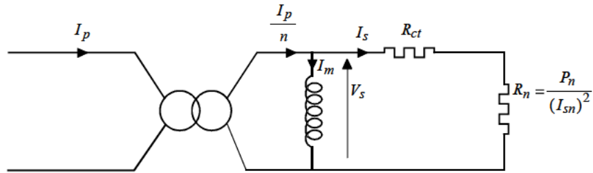
Figure 6-13: CT electrical diagram
