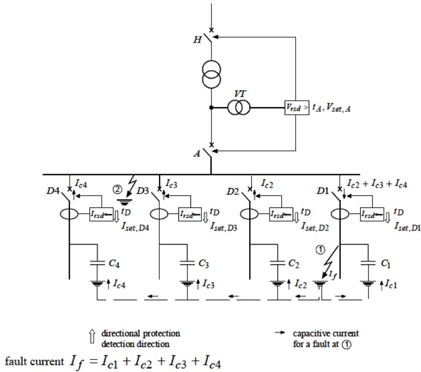
Figure 10-7: unearthed neutral
