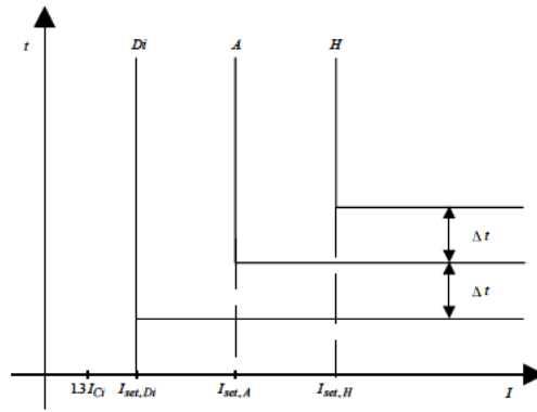
Figure 10-5b: selectivity curves
