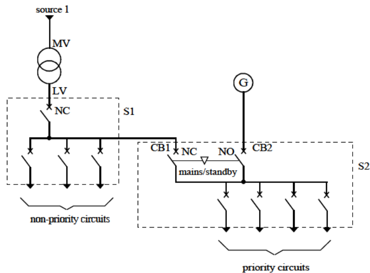
Figure 1-27: 1 transformer and 1 generator
