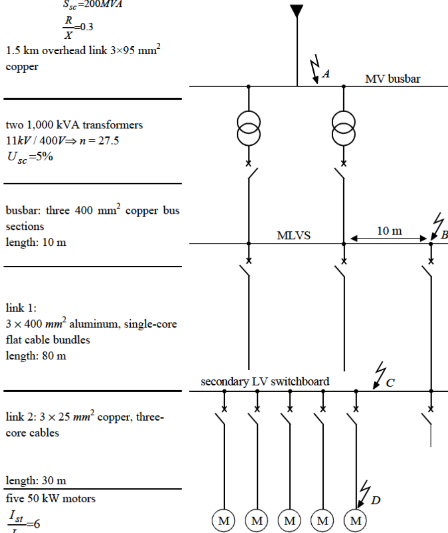
Figure 4-8: installation diagram for the symmetrical three-phase short-circuit calculation example
