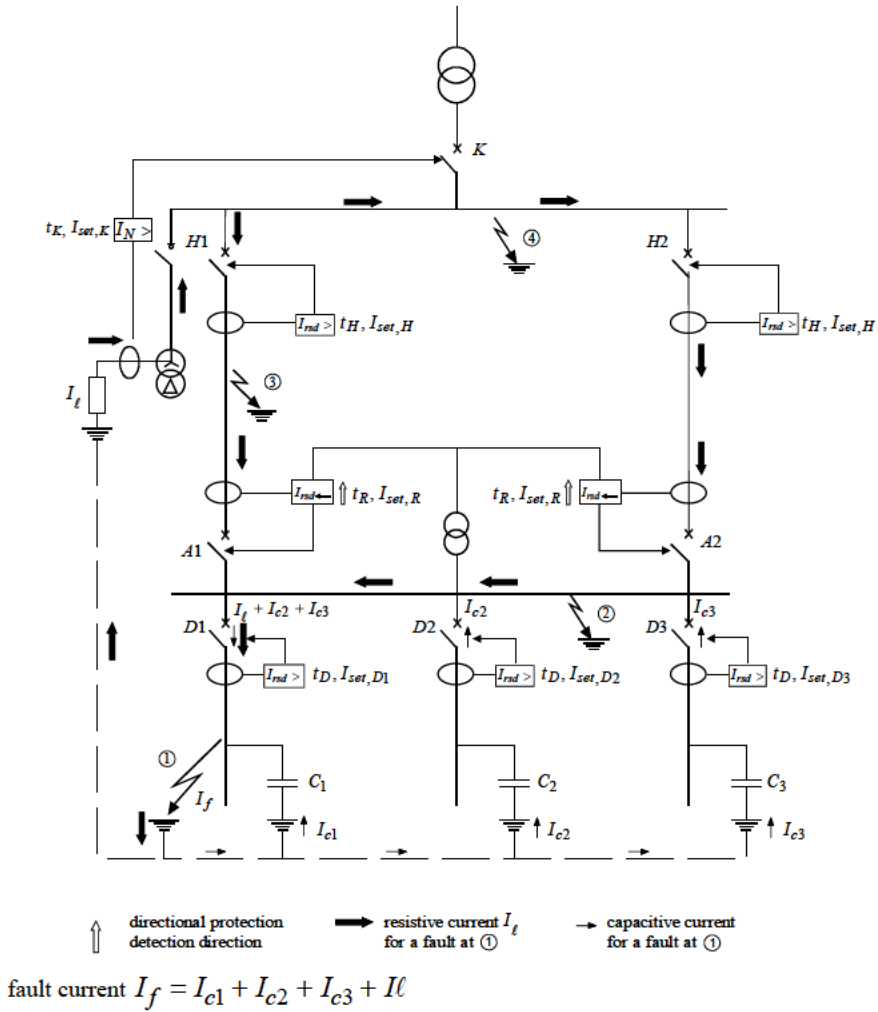
Figure 10-14: neutral earthing via resistance on the busbar
