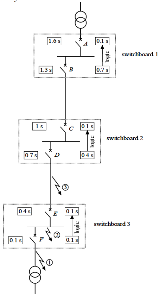
Figure 9-7: mixed selectivity
