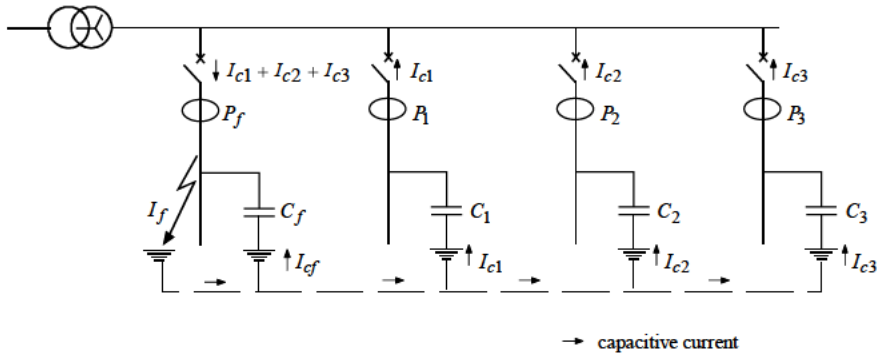
Figure 7-22: distinguishing between a fault current and a capacitive current in an ungrounded neutral system
