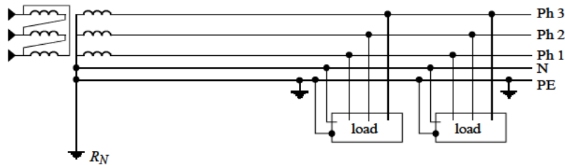
Figure 2-5: TNS system
