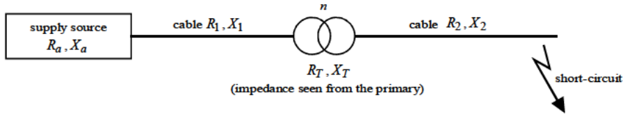
Figure 4-6: equivalent impedance of elements across a transformer
