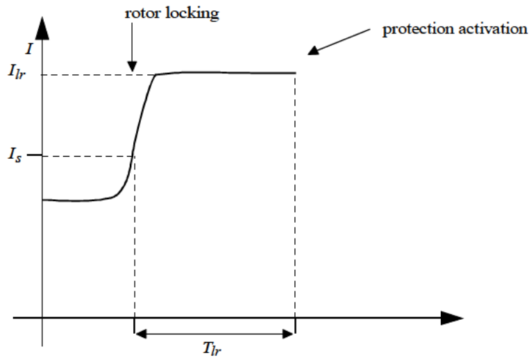
Figure 7-56: rotor locking
