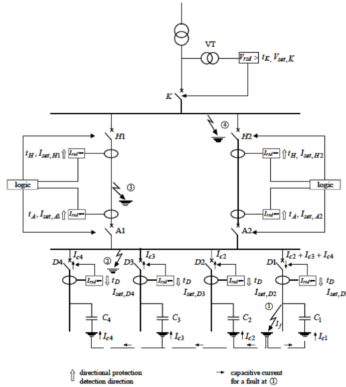
Figure 10-15: ungrounded neutral
