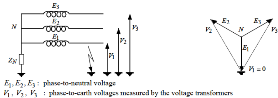
Figure 7-59: solid phase-to-earth fault in an unearthed or limiting impedance earthed system
