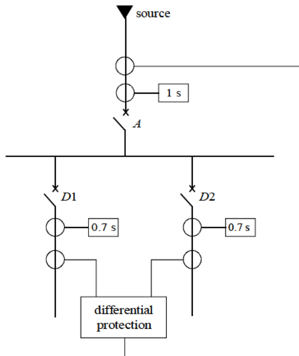
Figure 10-20c: protection of a busbar using a high impedance differential protection
